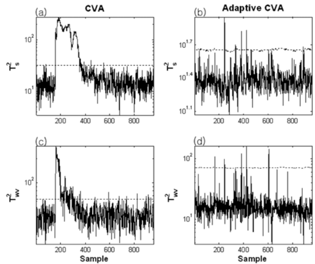
Fig. 7. The monitoring results for the TEP scenario 2 (CVA vs adaptive CVA).
