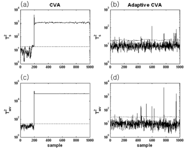
Fig. 3. Monitoring results for the CSTR scenario 2 (CVA vs adaptive CVA).
