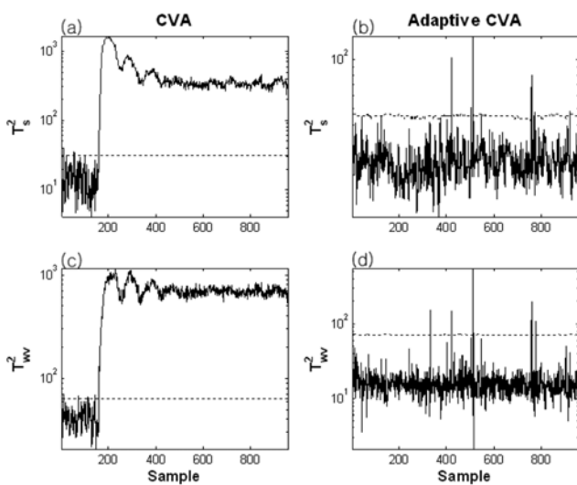
Fig. 5. Adaptive information of the TEP scenario 1 (CVA vs adaptive CVA).
