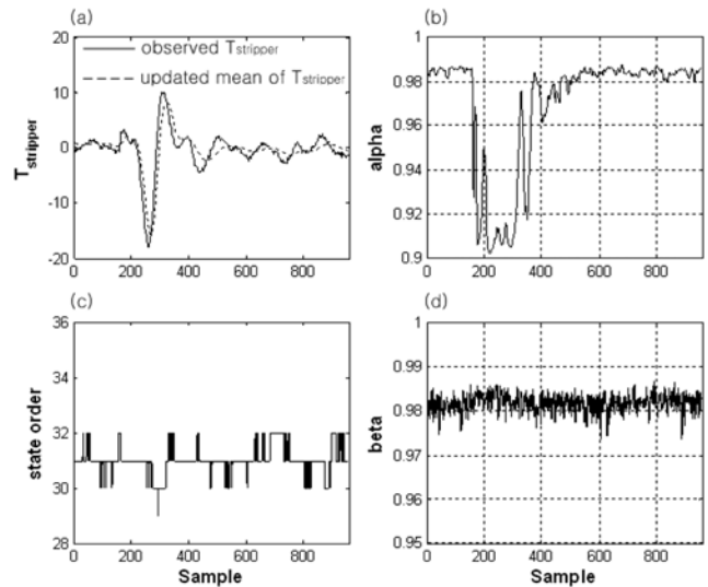
Fig. 8. Adaptive information of the TEP scenario 2.
