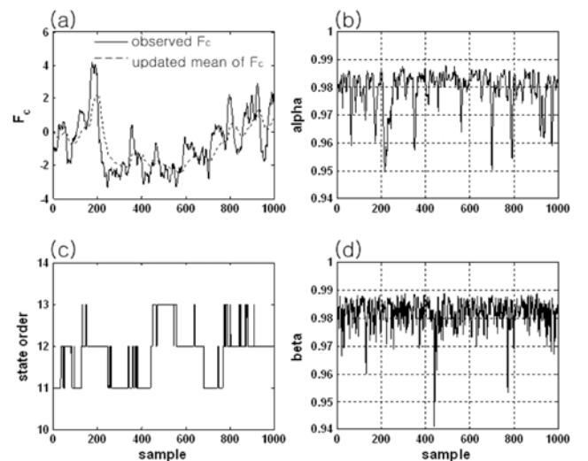
Fig. 4. Adaptive information of the CSTR scenario 2.
